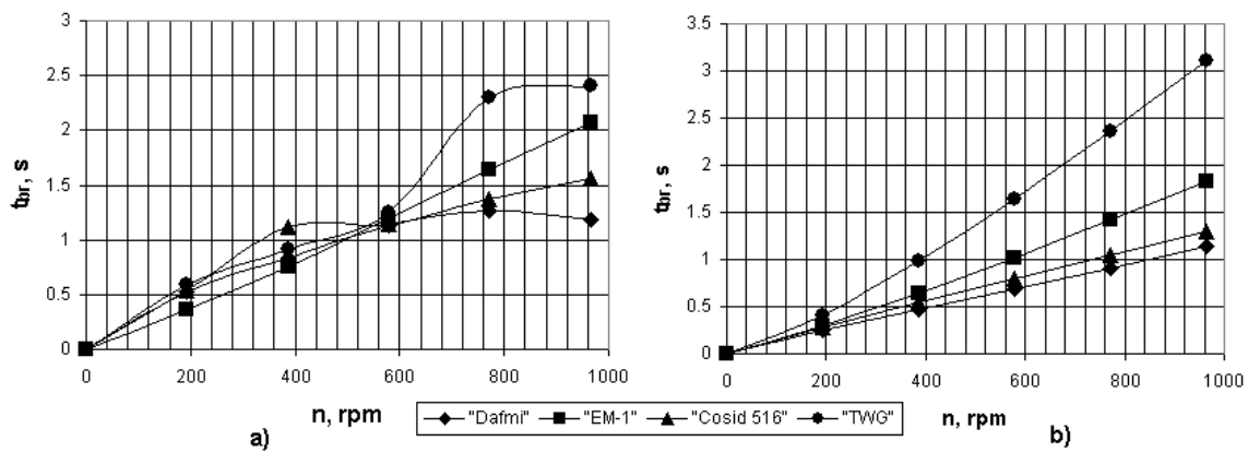
Fig. 4. The braking time t_{br} depending on a disc revolutions n at the beginning of braking ( p = 1.15 MPa, R = 2 time/min): a – results of experimental work; b – results of calculation
