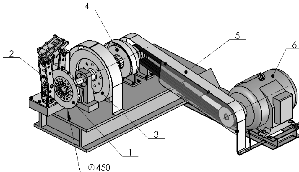
Fig. 1. Inertia stand: 1 – disc; 2 – disc brake DBE-1; 3 – flywheel; 4 – coupling (automatically unlink electromotor when necessary rotation speed is achieved); 5 – transmission with a cover; 6 – electromotor ( P = 45 kW)
