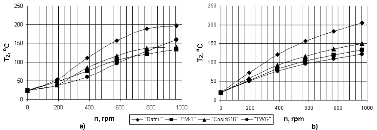
Fig. 2. The friction lining thermal balance temperature T_2 depending on a disc revolutions n at the beginning of braking ( p = 1.15 MPa, R = 2 time/min): a – results of experimental work; b – results of calculation
