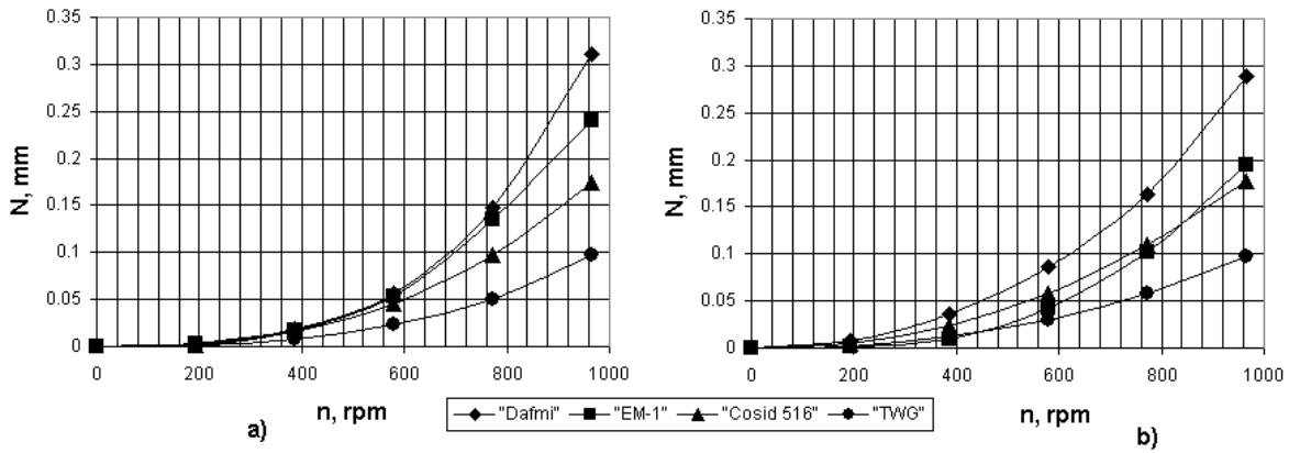
Fig. 3. The wear of friction lining N depending on a disc revolutions n at the beginning of braking ( p = 1.15 MPa, R = 2 time/min): a – results of experimental work; b – results of calculation
