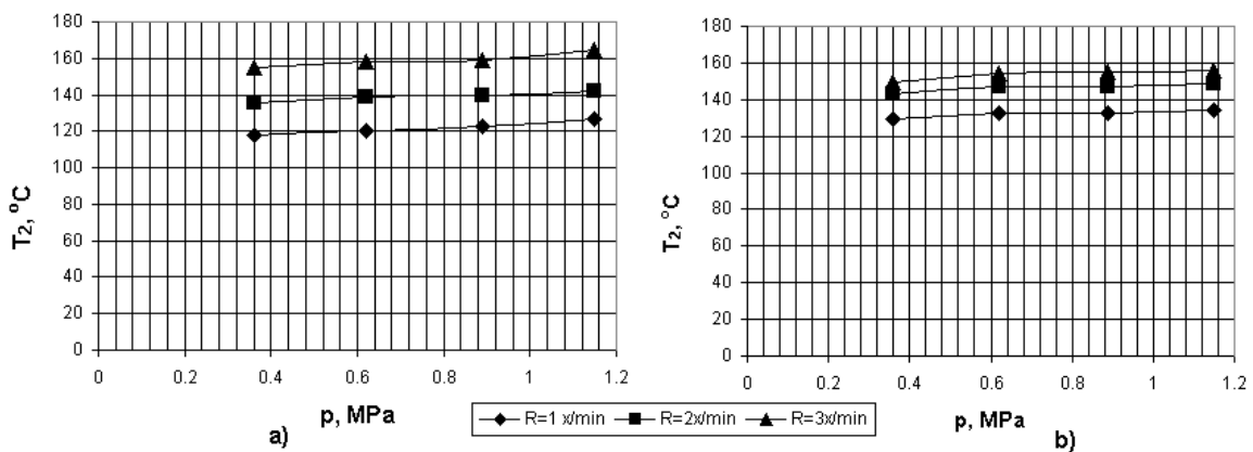
Fig. 5. The friction lining EM-1 thermal balance temperature T_2 depending on specific surface pressure p and braking intensity R ( p = 1.15 MPa, R = 2 time/min): a – results of experimental work; b – results of calculation
