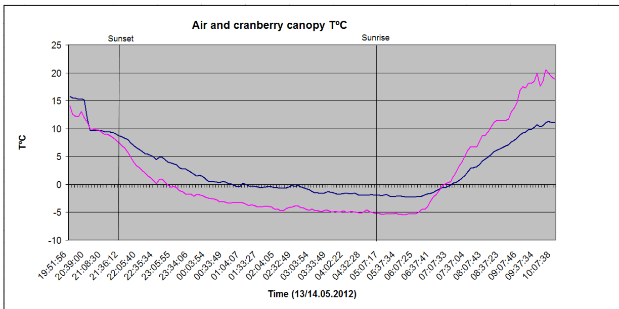
Fig. 3. Temperature curves.
