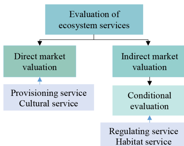
Fig. 4. Integrated valuation of ecosystem services considers.
