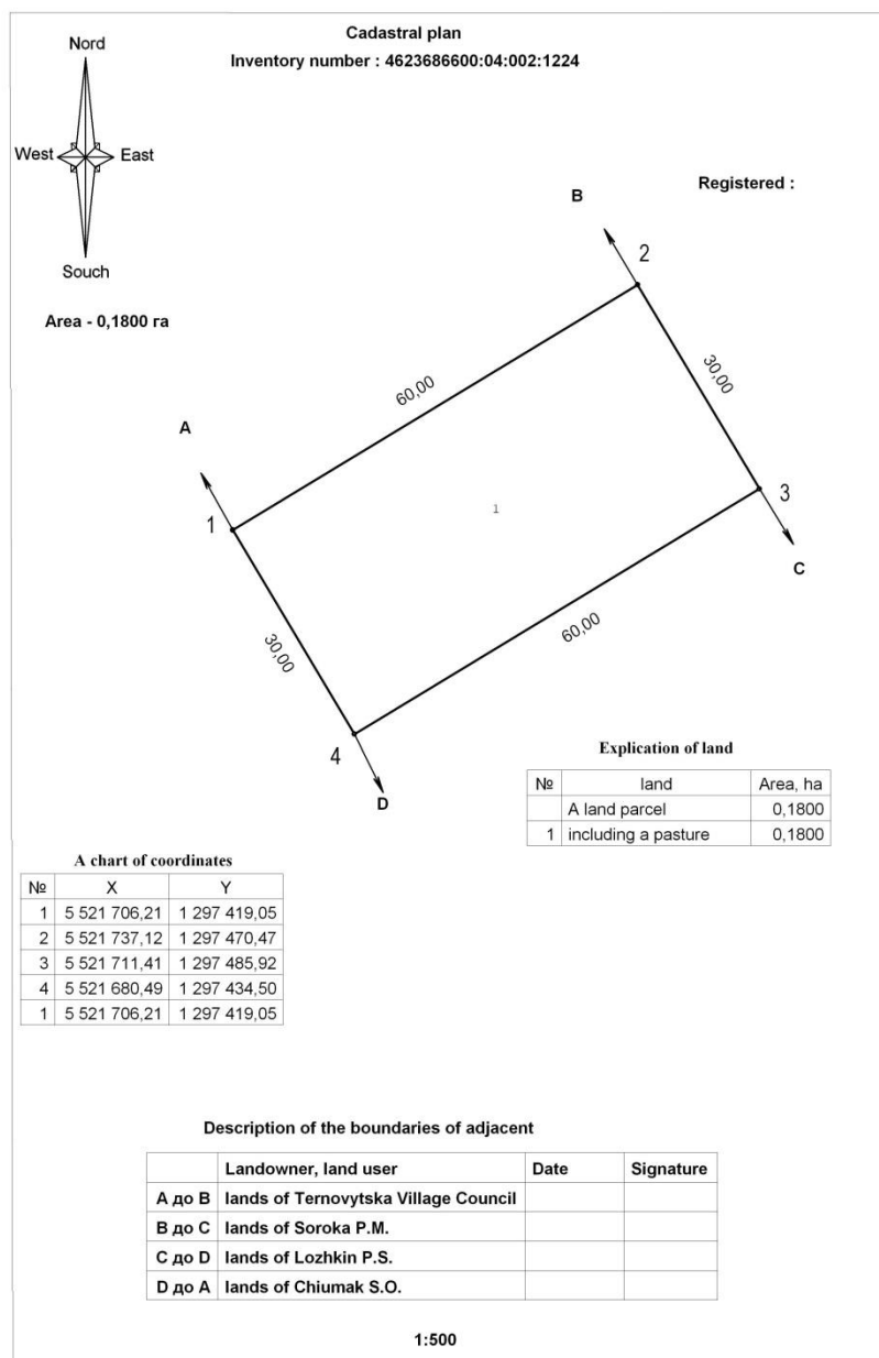
Fig.1. The cadastral plan of the land parcel.
