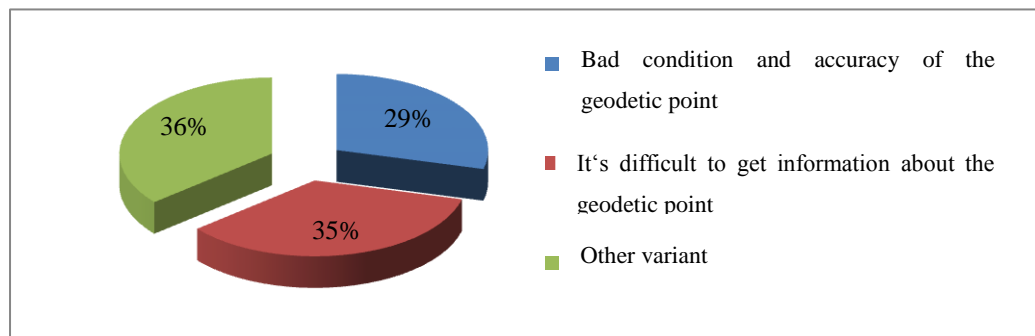
Fig. 4. The problems of usage of polygonometric points during land measurements.
