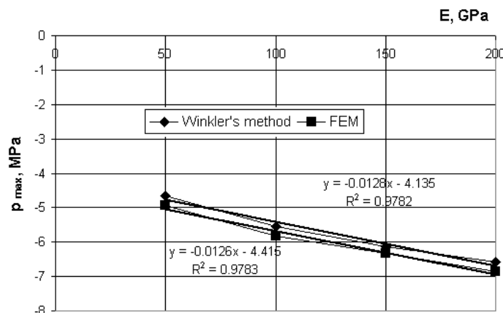
Fig. 8. The maximal specific surface pressure p_{max} depending on the module of friction lining elasticity E
