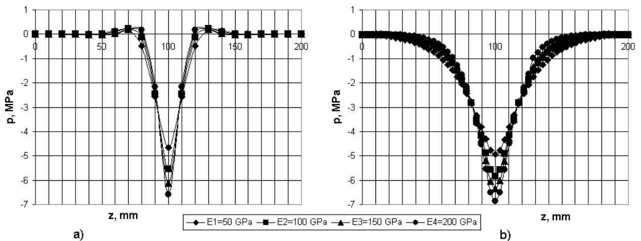
Fig. 5. The specific surface pressure p depending on resultant pressing force R in different split z of friction lining: a – using Winkler's method; b – using finite element method (FEM)
