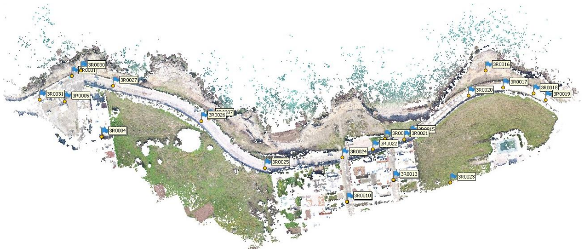
Fig. 3. Distribution of the GCPs implemented in the sparse points cloud
